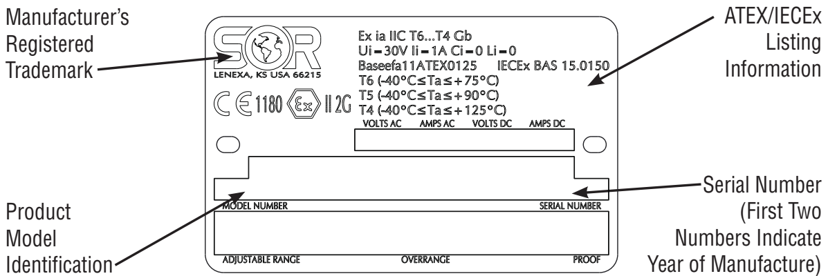
Drawing 0720044
